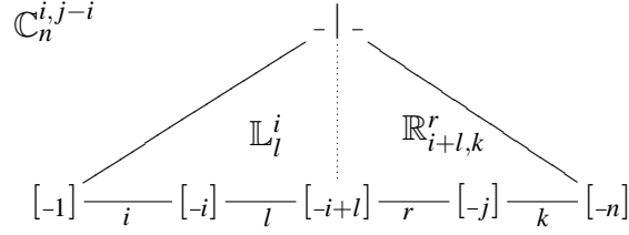
Figure 8. Synchronization contexts, graphically (where j = i + l + r and n = j + k ).
